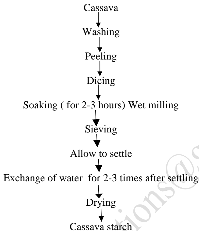
Fig 1 flow chart for production of cassava starch
